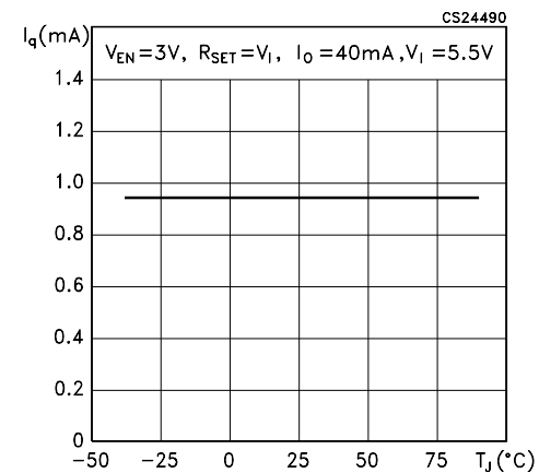
Figure 16. I_Q vs temperature
